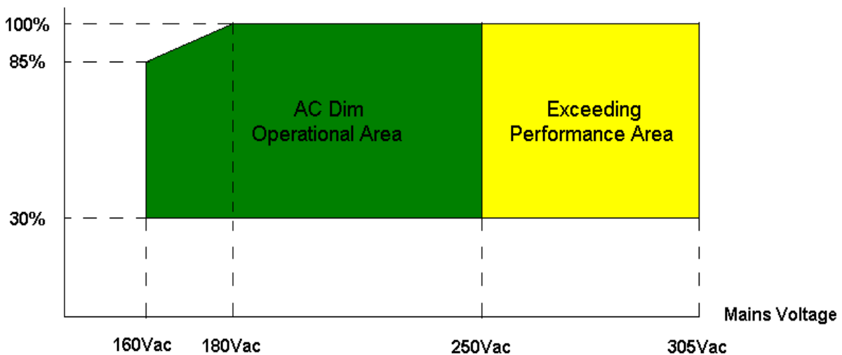
Output Level
