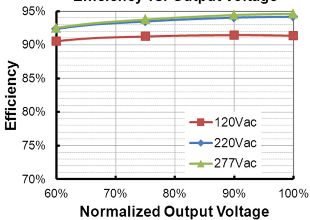
EUD-200S210DVA (Io=1400mA) Efficiency vs. Output Voltage
