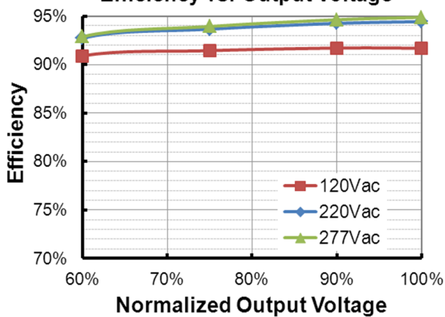
EUD-200S210DVA (Io=1400mA) Efficiency vs. Output Voltage
