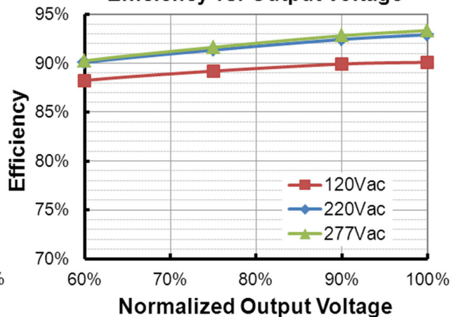
EUD-200S210DVA (Io=2100mA) Efficiency vs. Output Voltage
