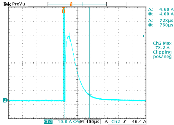
EBS-040S045BT2 (I o =300mA)
