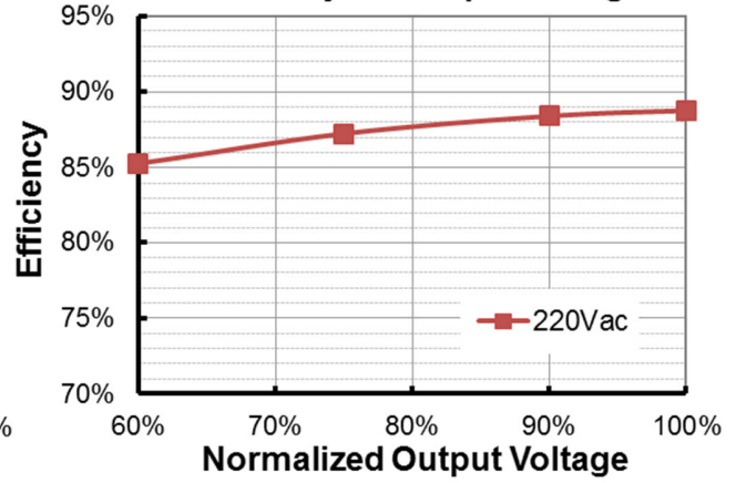
EBS-040S105BT2(Io=1050mA) Efficiency vs. Output Voltage
