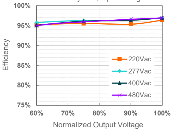
NFM-880S350Mx( I_o=1760mA ) Efficiency vs. Output Voltage
