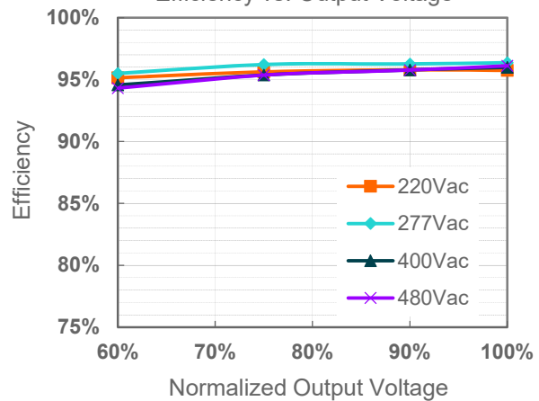
NFM-880S350Mx( I_o=3500mA ) Efficiency vs. Output Voltage
