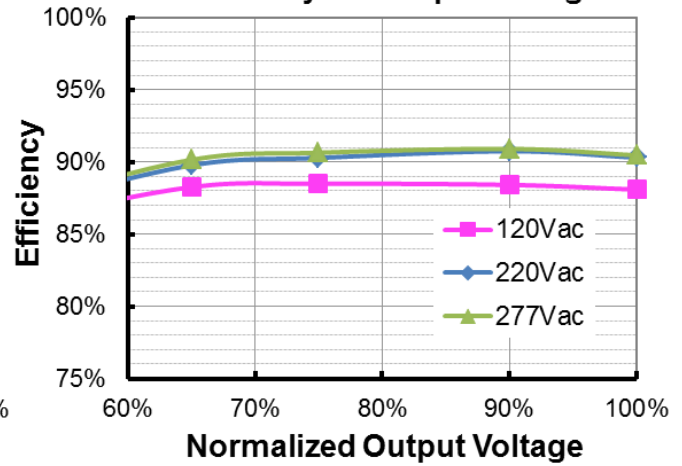
EUM-075S150Bx ( I_o=1500mA ) Efficiency vs. Output Voltage
