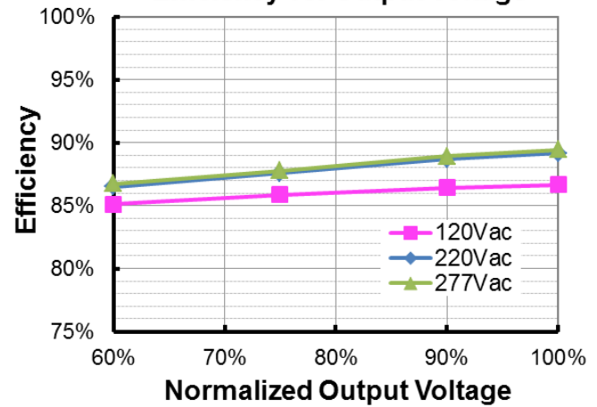
EUM-075S210Bx ( I_o=2100mA ) Efficiency vs. Output Voltage
